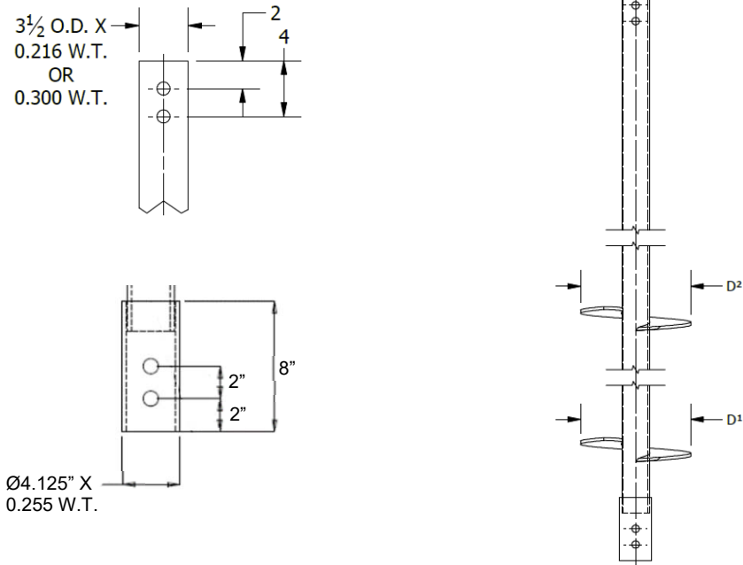
FIGURE 5B—TYPICAL 3 1/2-INCH-DIAMETER FLIGHTED EXTENSION
