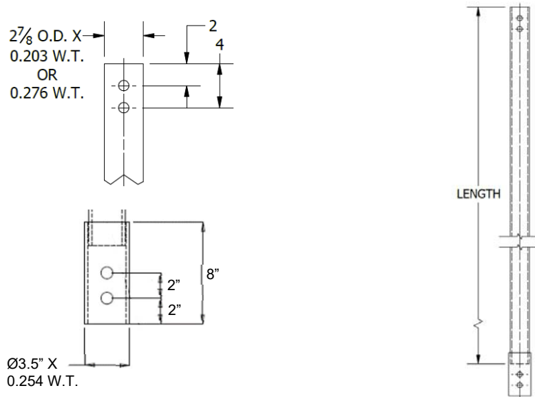
FIGURE 3A—TYPICAL 2 7/8-INCH-DIAMETER EXTENSION SHAFT SECTION
